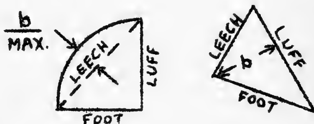
Sail measurement for handicap rule used by the Eastern Multihull Sailing Association
